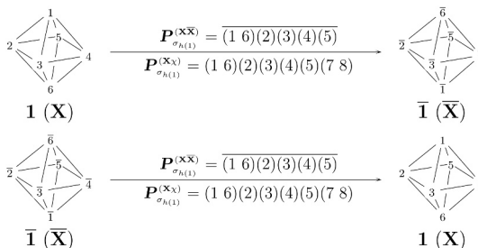
Figure 3. Reflections for an Octahedral Skeleton
