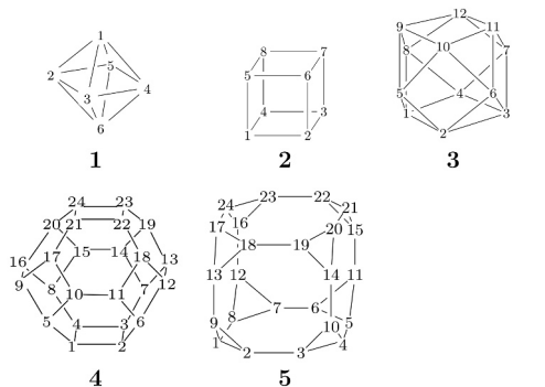
Figure 1. O_h -Skeletons: Octahedron 1 ( OC-6 ), cube 2 ( CU-8 ), 3 , truncated octahedron 4 , and truncated hexahedron (truncated cube) 5 .
