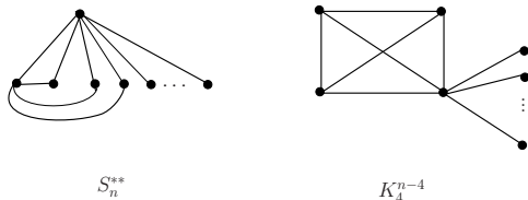
Figure 1: Tricyclic graphs with minimal matching energy.
