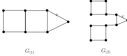
Figure 3: The fundamental graphs for constructing G_{(1)}^n and G_{(2)}^n .
