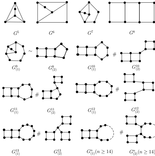
Figure 2: The tricyclic graphs with a maximal number of matchings.
