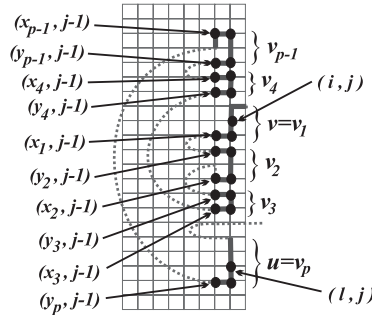
Figure 6: Property (3c) of modified code matrix
