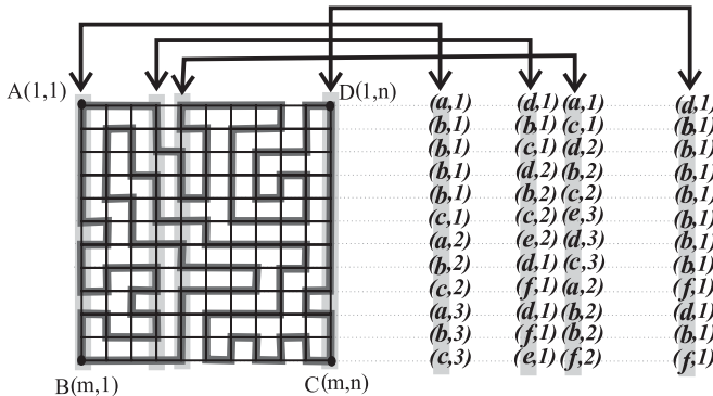
Figure 4: Coding vertices of graph P_m \times P_n
