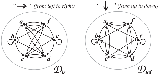
Figure 3: Left-right and up-down adjacency of two vertices
