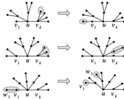
Figure 3: Tree transformations from Lemmas 6, 7 and 8 respectively.
