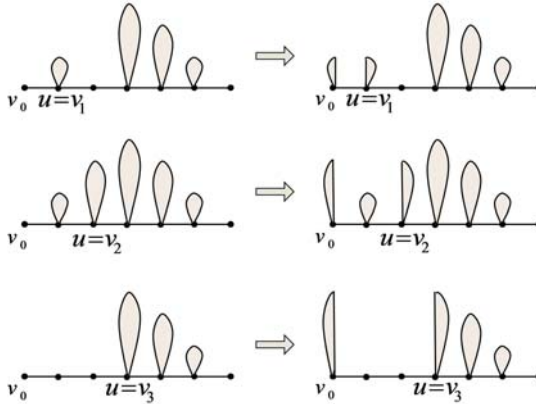
Figure 2: Tree transformations from Cases 1, 2 and 3 of Theorem 2.
