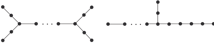
Figure 1. Trees T_n(2, 2|2, 2) and P_n(2, 6, n-9) .
