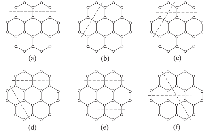
Figure 3: Types of pairs of cuts in the coronene
