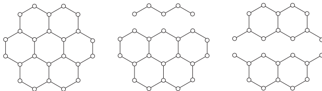
Figure 2: Coronene H_2 and two of its cuts
