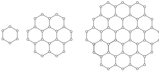
Figure 1: The first three graphs, H_1 , H_2 , and H_3 , from the circumcoronene series
