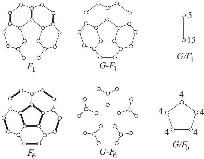
Figure 4: Computing the Wiener index of C_{20}(2)
